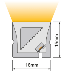
Product dimensions
