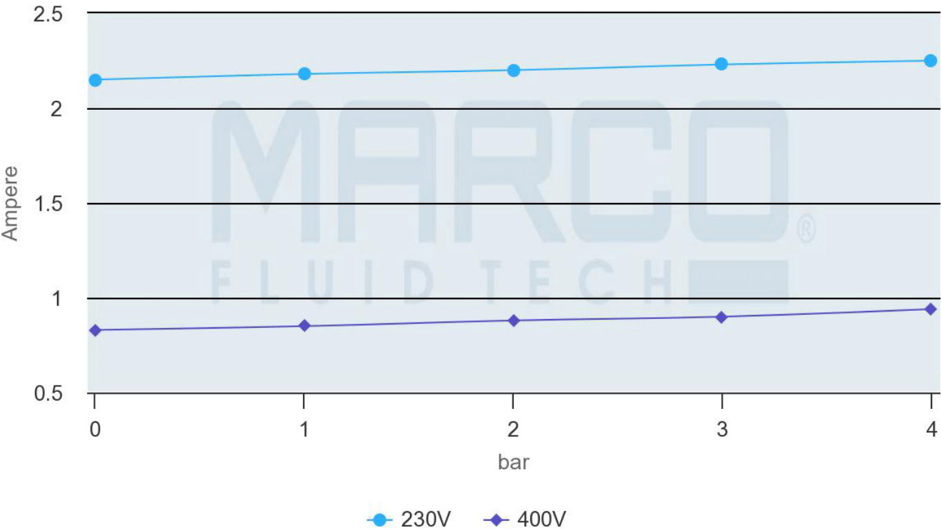
Electrical absorption UP14-OIL-AC
