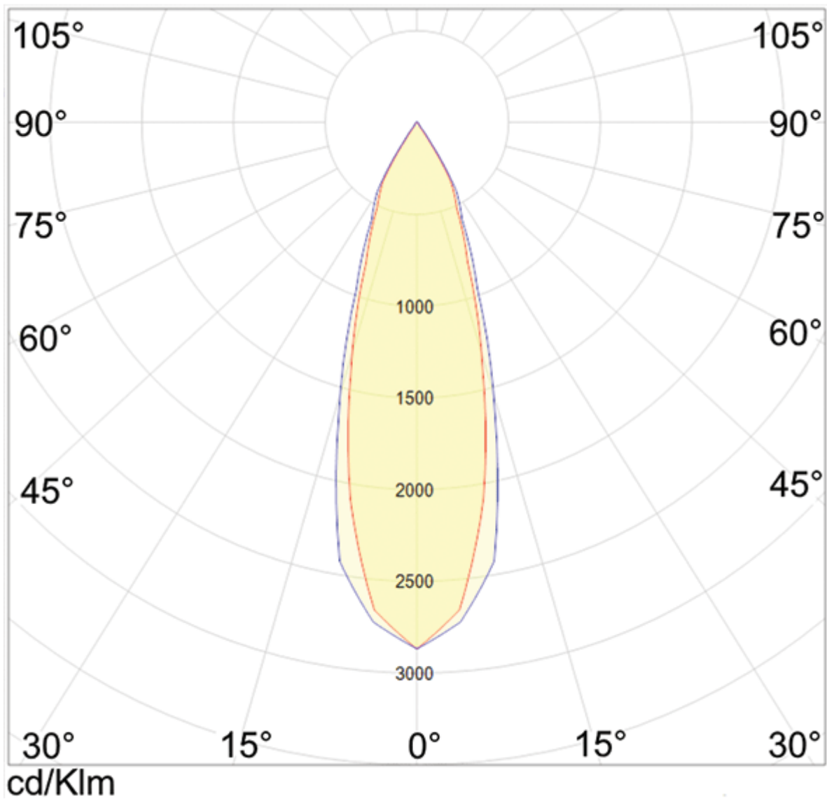
5270 - 29° Lens (.9M)
