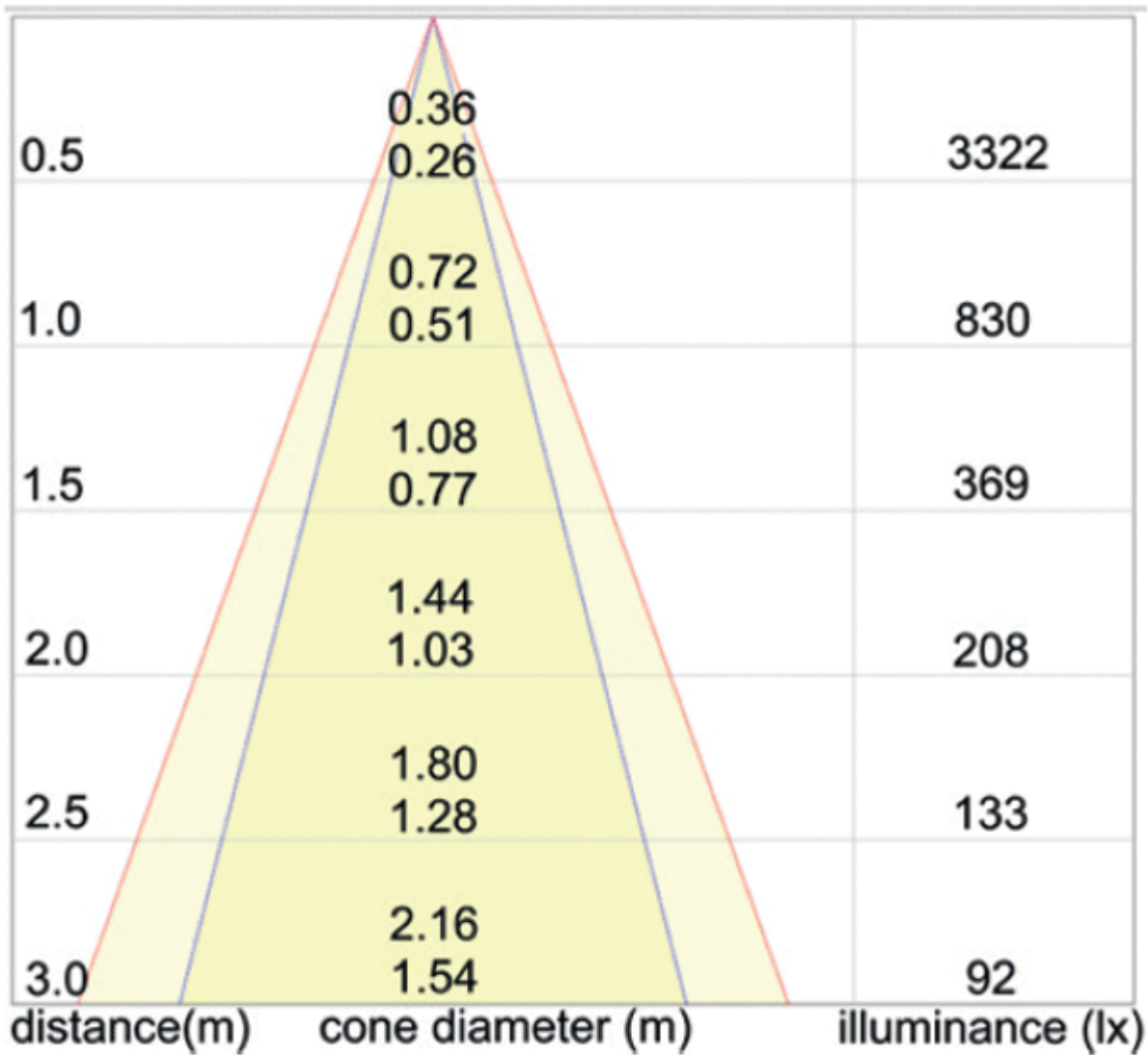
5271 - 43-24° Elliptical Lens (.9EL)
