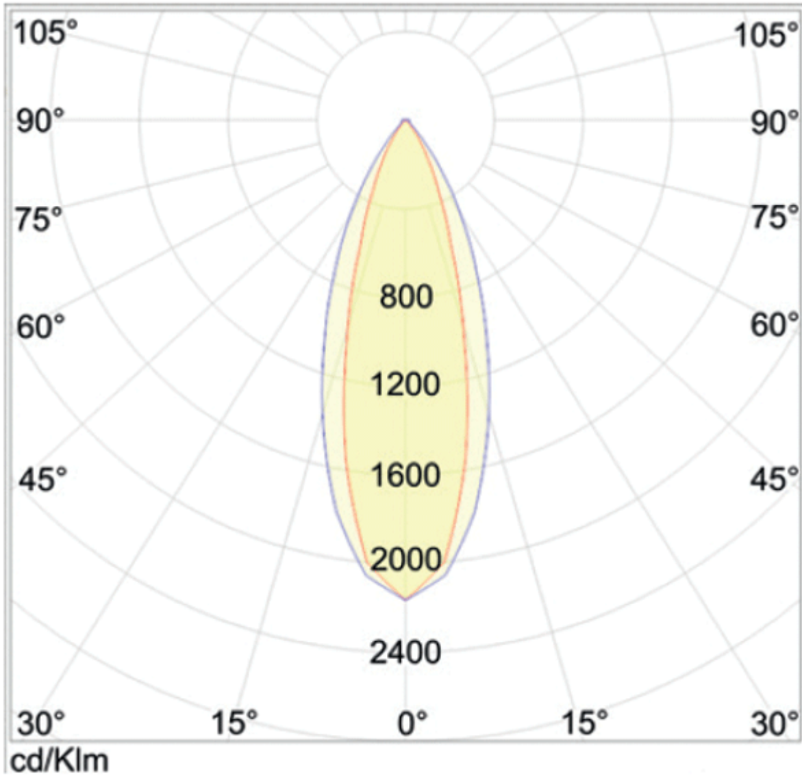
5292 - 21-14° Elliptical Lens (.9EL)
