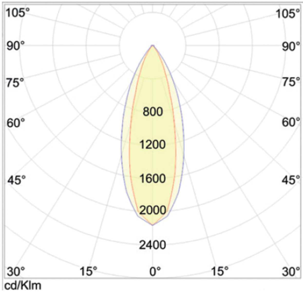
5292 - 21-14° Ellipitcal Lens (.9EL)
