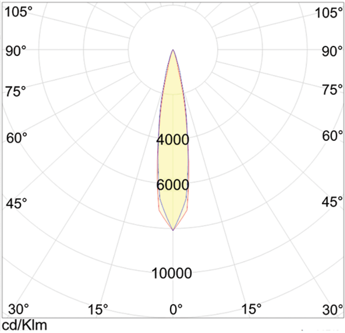
5277 - 13° Lens (.9N)
