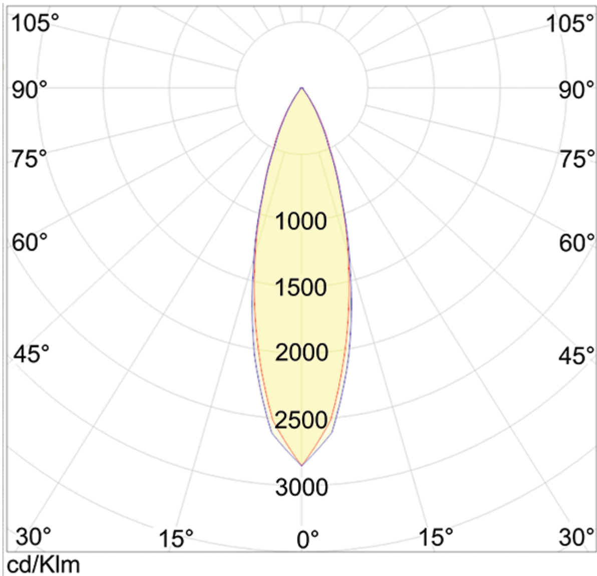
5277 - 23° Lens (.9M)
