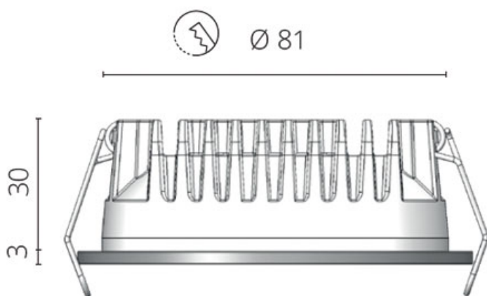
Power Led
