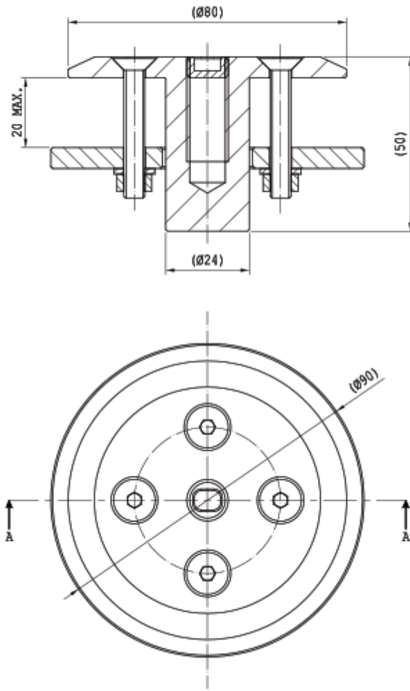
IC-IP4501SS Fixing From Underneath
