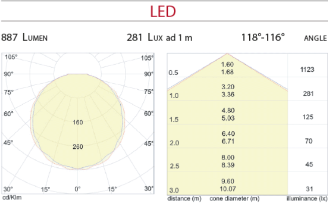
RIGHT LINE E art./ref. 8390.L6 / 8391.L6
