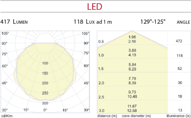
RIGHT LINE E art./ref. 8390.L2 / 8391.L2
